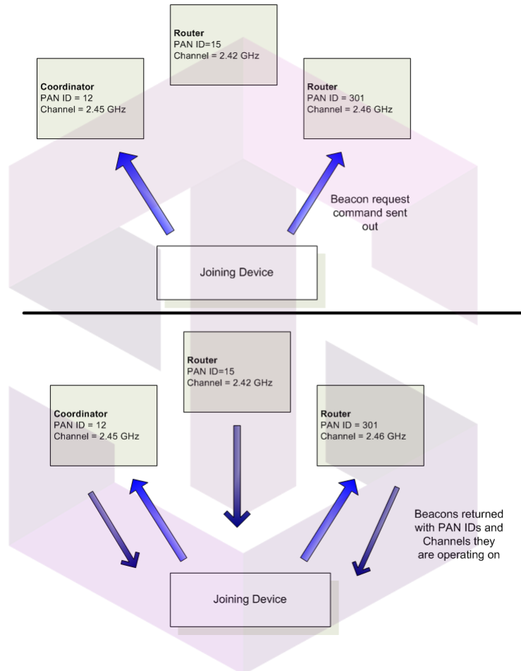
Figure 3-02. Demonstration of Beacon Request and Beacon transmissions that take place during joining.
